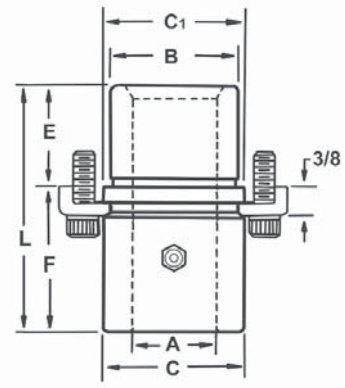
STANDARD SHOULDER
